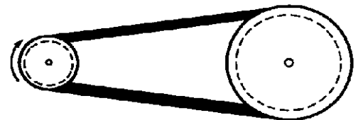
ENGINE DRIVE PULLEY 10,000 RPM \pm 500 RPM = 4750-5250 RPM WHEEL SPEED
